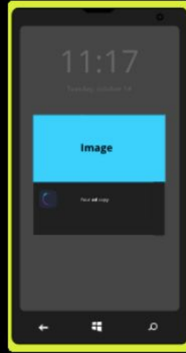
Windows
